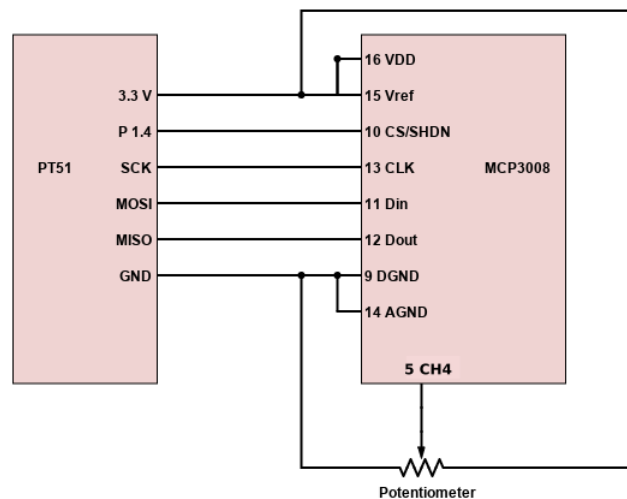
Figure 1: Pt51 interfacing with ADC and potential divider.
